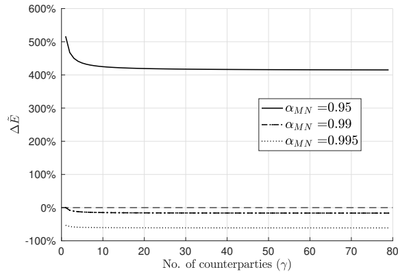
(a) Change in exposure due to cross-netting across \kappa = 10 derivative classes.
