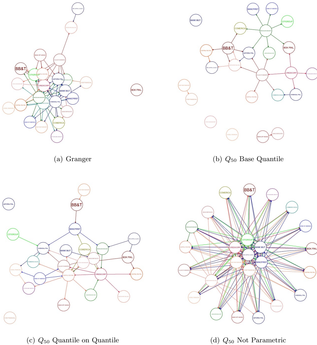
Figure C.10: This figure visualizes 4 different networks for the period 2006–2008 relative to the first 25 banks ordered for market capitalization. In this case the networks visualized are some of the primitive networks used for the resulting network computations. Panel a) reports the network extracted by the standard granger causality. Panel b) indicates the network extracted by a quantile baseline regression methodology on the 50% quantile q_{50} . Panel c) indicates the network extracted by a quantile on quantile methodology on the 50% quantile q_{50} . Panel d) reports the network extracted by a not parametric methodology on the 50% quantile q_{50} . All the causality regression are computed without the market factor.
