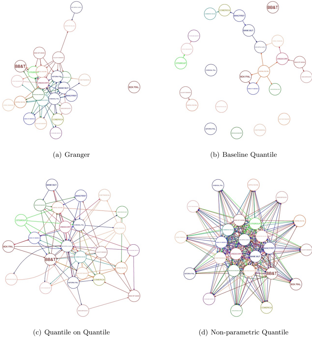
Figure 2: The figure visualizes 4 different networks for the period 2006-2008 relative to the first 25 banks ordered for market capitalization and listed in Appendix A. Panel a) reports the network extracted by the standard Granger causality approach of (Billio et al., 2012). Panel b) reports the Network extracted from a baseline quantile regression methodology, at the 10% quantile. Panel c) plots the network extracted from a quantile-on-quantile methodology at the 10% quantile. Panel d) graphs the network estimated by a non-parametric quantile causality methodology at the 10% quantile. All the estimates exclude the presence of common factors. We use the Fruchterman & Reingold algorithm for network visualization.
