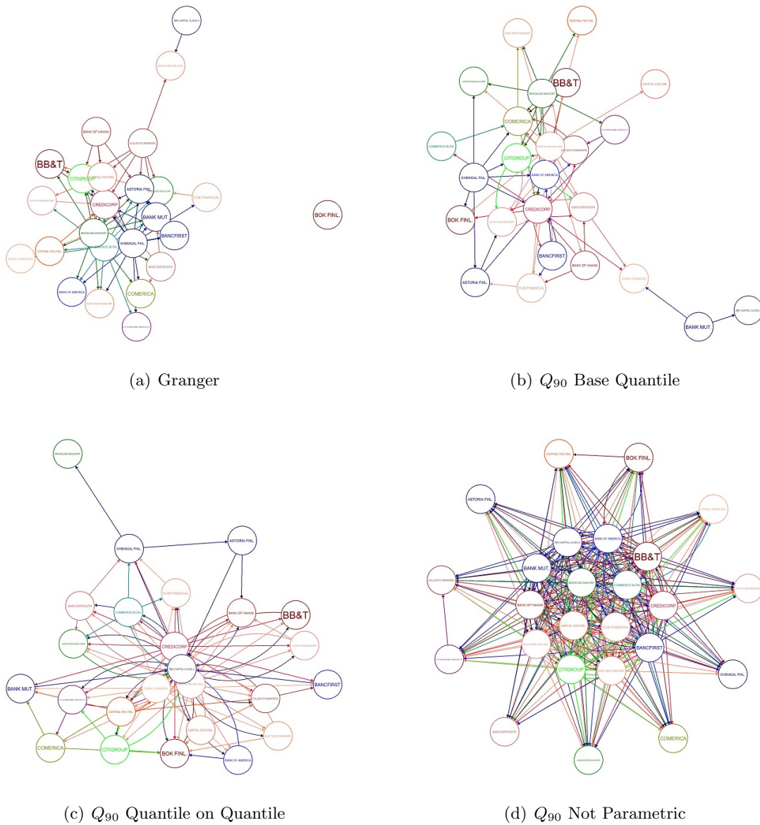
Figure C.11: This figure visualizes 4 different networks for the period 2006–2008 relative to the first 25 banks ordered for market capitalization. In this case the networks visualized are some of the primitive networks used for the resulting network computations. Panel a) reports the network extracted by the standard granger causality. Panel b) indicates the network extracted by a quantile baseline regression methodology on the 90% quantile q_{90} . Panel c) indicates the network extracted by a quantile on quantile methodology on the 90% quantile q_{90} . Panel d) reports the network extracted by a not parametric methodology on the 90% quantile q_{90} . All the causality regression are computed without the market factor.
