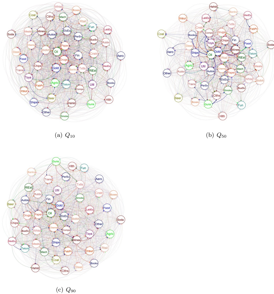
Figure E.25: This figure visualizes the 3 different resulting networks for the period 2006-2008 relative to 48 Industry portfolios. Panel a) reports the network extracted by combining causality network by using quantile regression (QB, Q_0 and Q_N ) at the 10% quantile, and the standard granger causality method. Panel b) reports the network extracted by combining causality network by using quantile regression (QB, Q_0 and Q_N ) at the 50% quantile, and the standard granger causality method. Panel c) reports the network extracted by combining causality network by using quantile regression (QB, Q_0 and Q_N ) at the 90% quantile, and the standard granger causality method. All the causality regression are computed without the market factor.
