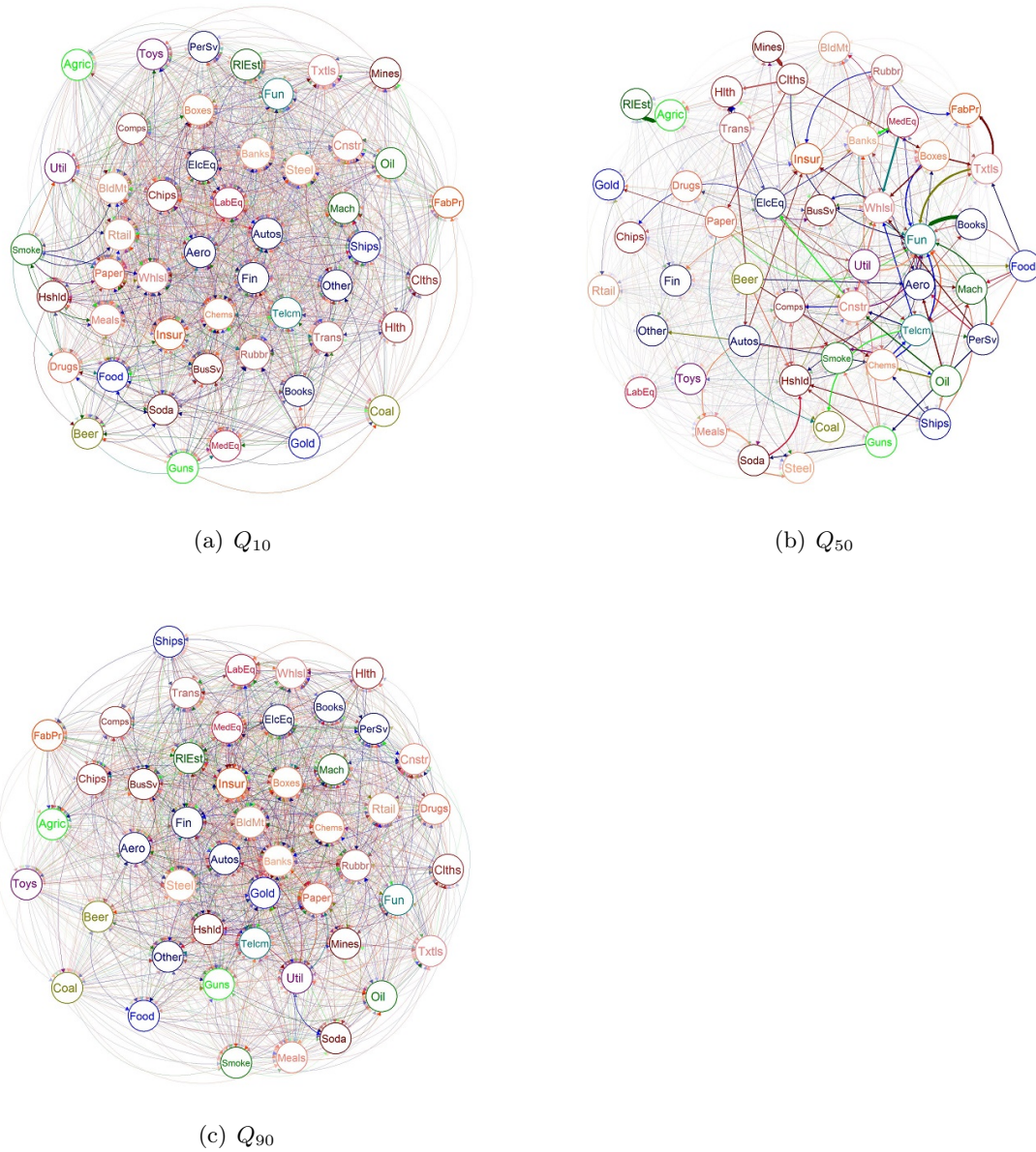
Figure E.26: This figure visualizes the 3 different resulting networks for the period 2011-2015 relative to 48 Industry portfolios. Panel a) reports the network extracted by combining causality network by using quantile regression (QB, Q_0 and Q_N ) at the 10% quantile, and the standard granger causality method. Panel b) reports the network extracted by combining causality network by using quantile regression (QB, Q_0 and Q_N ) at the 50% quantile, and the standard granger causality method. Panel c) reports the network extracted by combining causality network by using quantile regression (QB, Q_0 and Q_N ) at the 90% quantile, and the standard granger causality method. All the causality regression are computed without the market factor.
