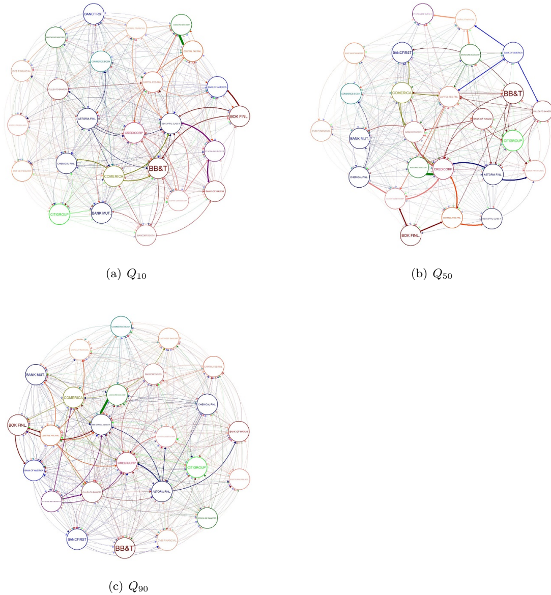
Figure E.21: This figure visualizes the 3 different resulting networks for the period 2006-2008 relative to the first 25 banks ordered for market capitalization. Panel a) reports the network extracted by combining causality network by using quantile regression (QB, Q_0 and Q_N ) at the 10% quantile, and the standard granger causality method. Panel b) reports the network extracted by combining causality network by using quantile regression (QB, Q_0 and Q_N ) at the 50% quantile, and the standard granger causality method. Panel c) reports the network extracted by combining causality network by using quantile regression (QB, Q_0 and Q_N ) at the 90% quantile, and the standard granger causality method. All the causality regression are computed without the market factor.
