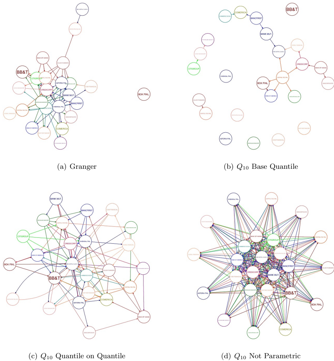
Figure C.9: This figure visualizes 4 different networks for the period 2006–2008 relative to the first 25 banks ordered for market capitalization. In this case the networks visualized are some of the primitive networks used for the resulting network computations. Panel a) reports the network extracted by the standard granger causality. Panel b) indicates the network extracted by a quantile baseline regression methodology on the 10% quantile q_{10} . Panel c) indicates the network extracted by a quantile on quantile methodology on the 10% quantile q_{10} . Panel d) reports the network extracted by a not parametric methodologie on the 10% quantile q_{10} . All the causality regression are computed without the market factor.
