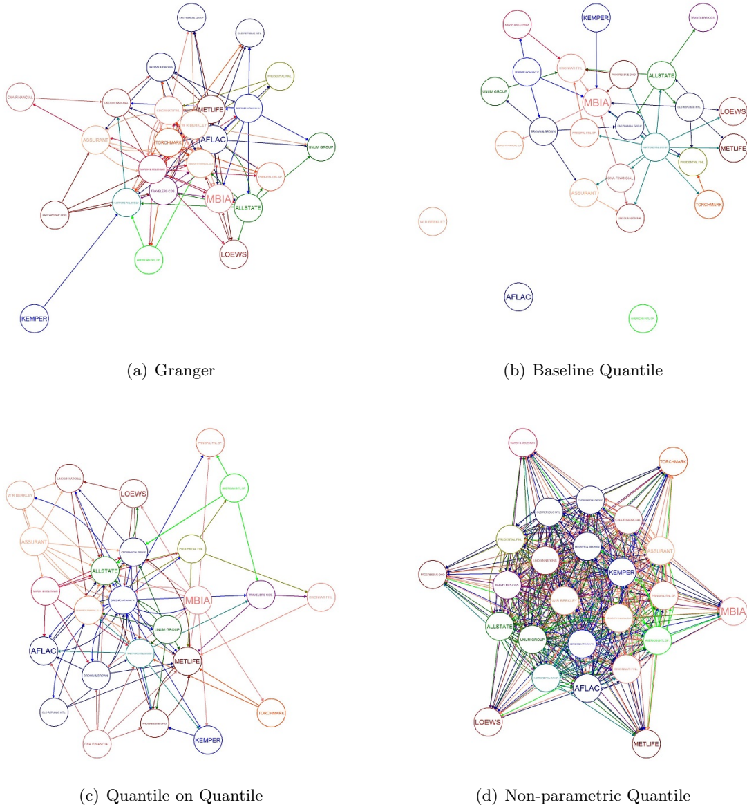
Figure 3: The figure visualizes 4 different networks for the period 2006-2008 relative to the first 25 insurances ordered for market capitalization and listed in Appendix A. Panel a) reports the network extracted by the standard Granger causality approach of (Billio et al., 2012). Panel b) reports the Network extracted from a baseline quantile regression methodology, at the 10% quantile. Panel c) plots the network extracted from a quantile-on-quantile methodology at the 10% quantile. Panel d) graphs the network estimated by a non-parametric quantile causality methodology at the 10% quantile. All the estimates exclude the presence of common factors. We use the Fruchterman & Reingold algorithm for network visualization.
